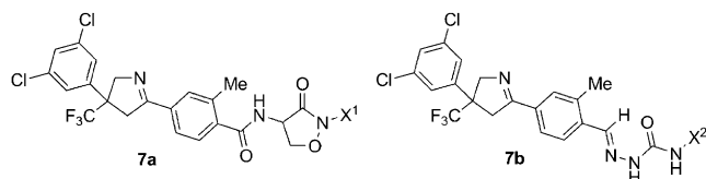
Figure 3. Agrochemically important trifluoromethylated pyrrolines 7.
