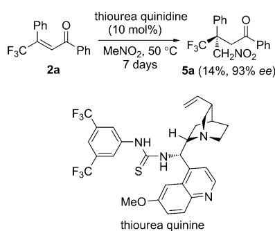
Scheme 1. The conjugate addition of nitromethane to 2a using cinchona alkaloid/thiourea catalyst.
